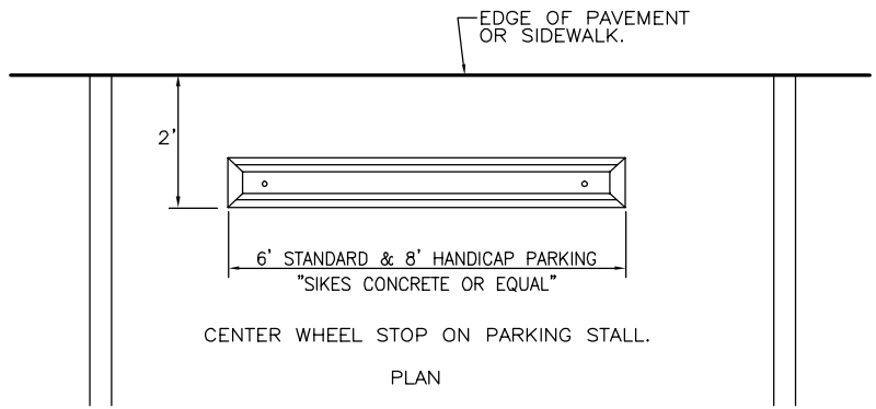
WHEEL STOP DETAIL NOT TO SCALE
