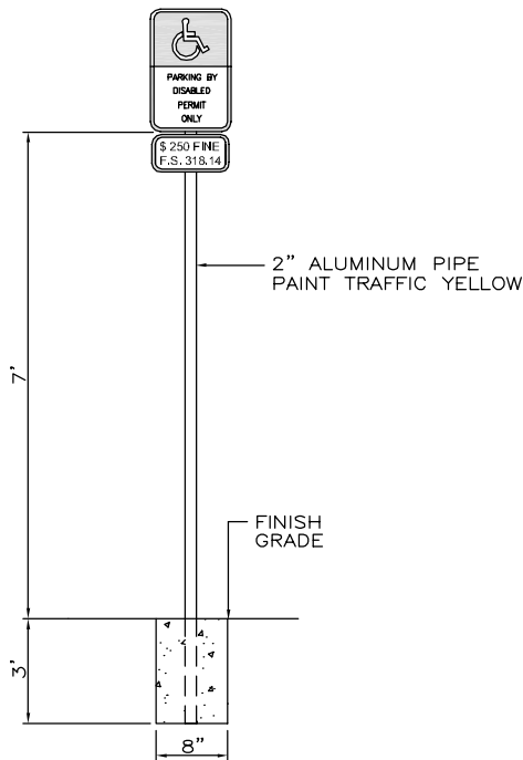
HANDICAP SIGN DETAIL NOT TO SCALE
